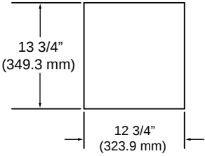
[D] - 3/4" (19 mm) MDF
